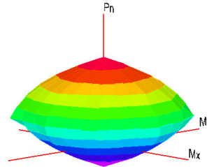
360 Degree P-M Curve 3D Envelope
