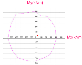
My/Mx Curve
