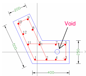
V-Shape Column
