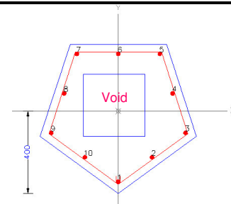
Equal Polygon Column
