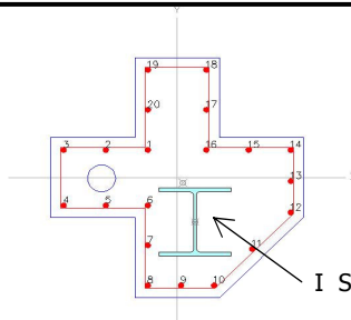
User Defined Composite Column
