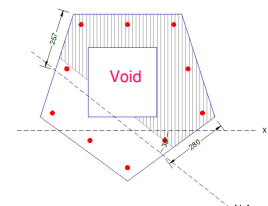
Neutral Axis Diagram
